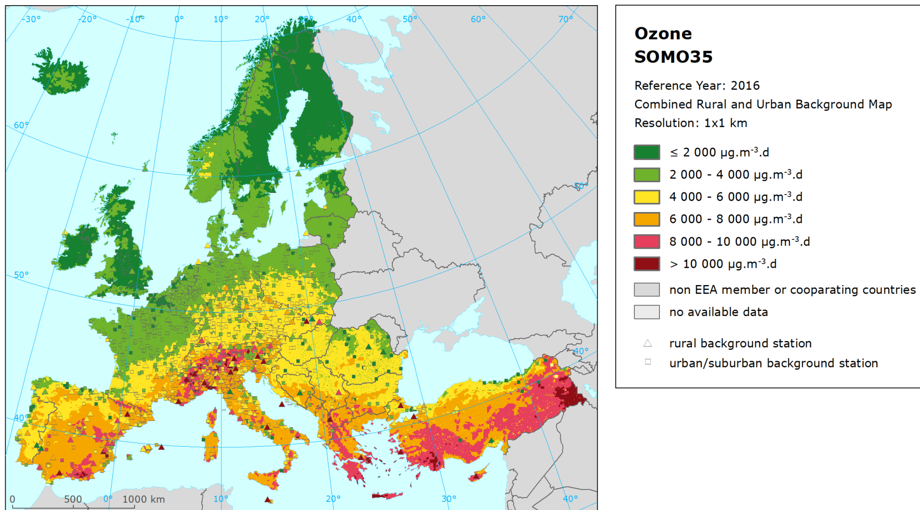
Map A5.5 Concentration map of ozone indicator SOMO35 including station points, 2016
