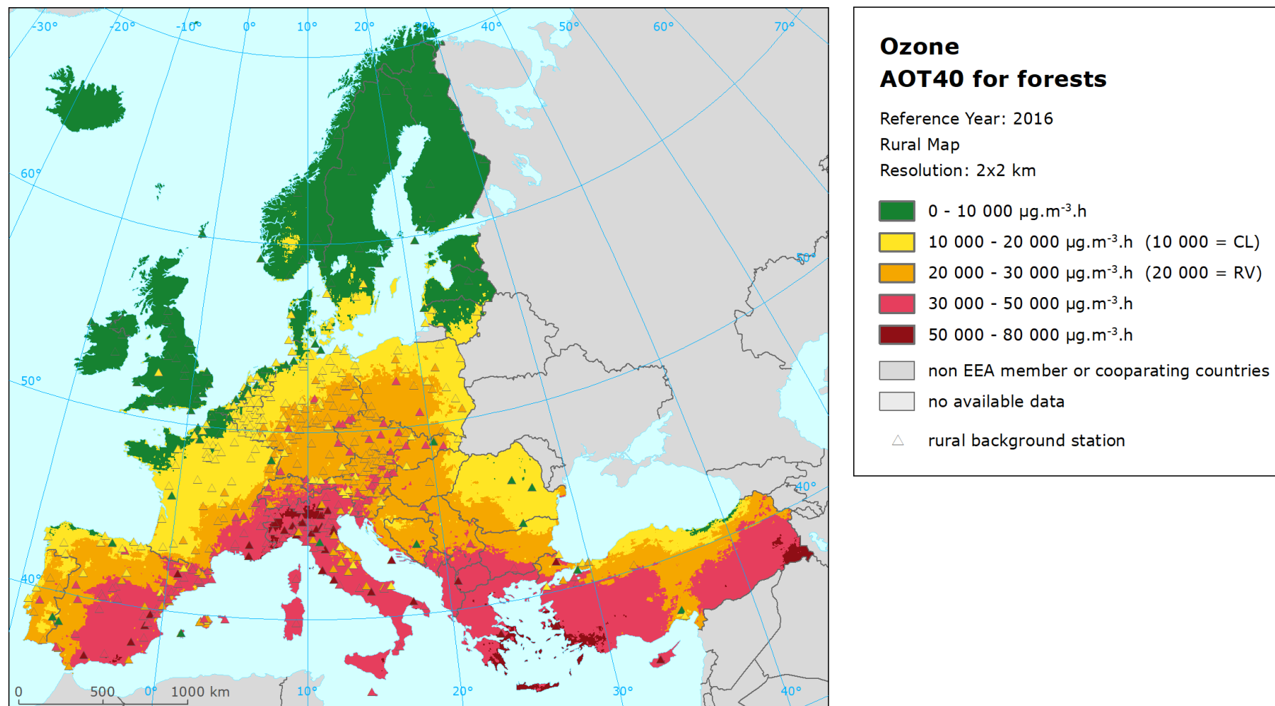
Map A5.7 Concentration map of ozone indicator AOT40 for forests including station points, rural air quality, 2016
