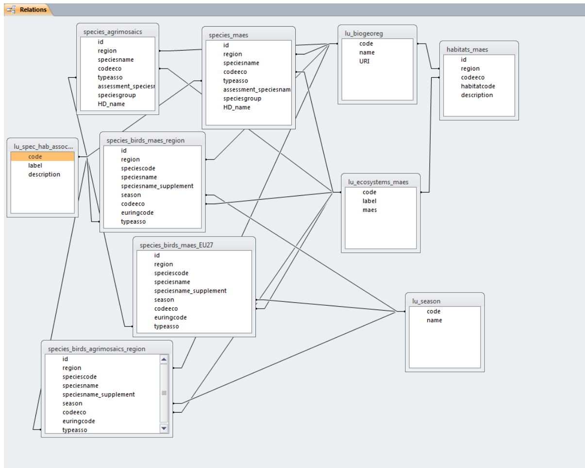
Figure 3-1 Entity Relationship diagram
