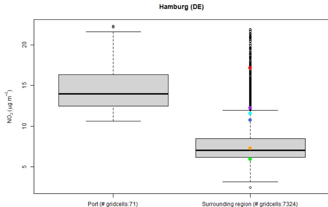
Concentrations over the port area compared to the surrounding region. Coloured dots correspond to weighted area means for different land cover classes in the surrounding region.
