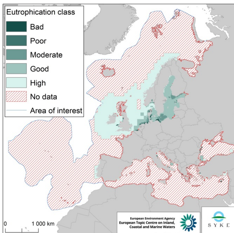
Figure 3.17: Integrated assessment of eutrophication in Europe's marine area. In the southern sea areas the assessment is done for coastal waters (not properly visible). See Appendix A for the data layer description.
