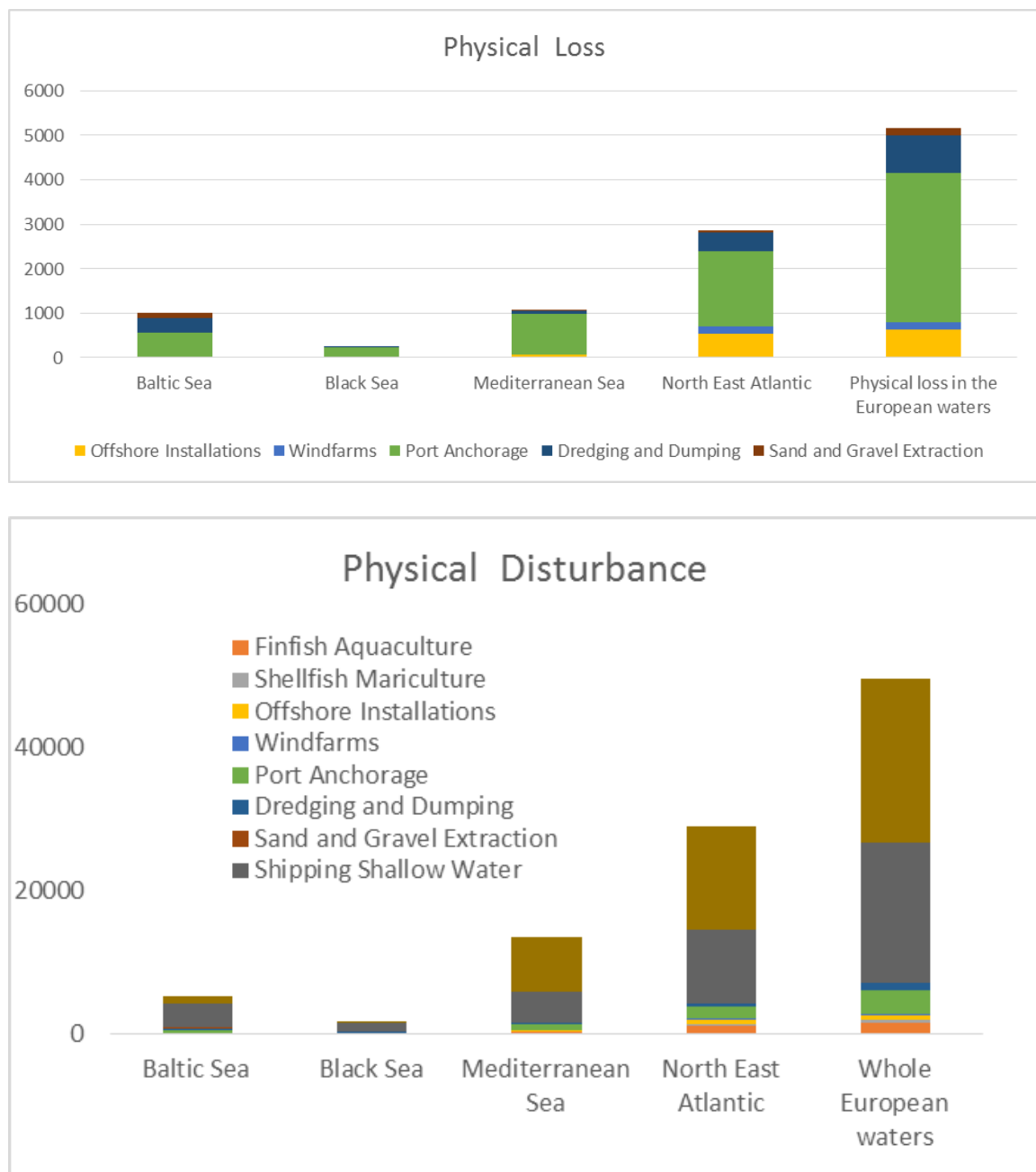
Figure 3.24: Seabed area (km 2 ) estimated as physically lost (A) or potentially disturbed (B). The area is also divided between different causes of loss and disturbance.
